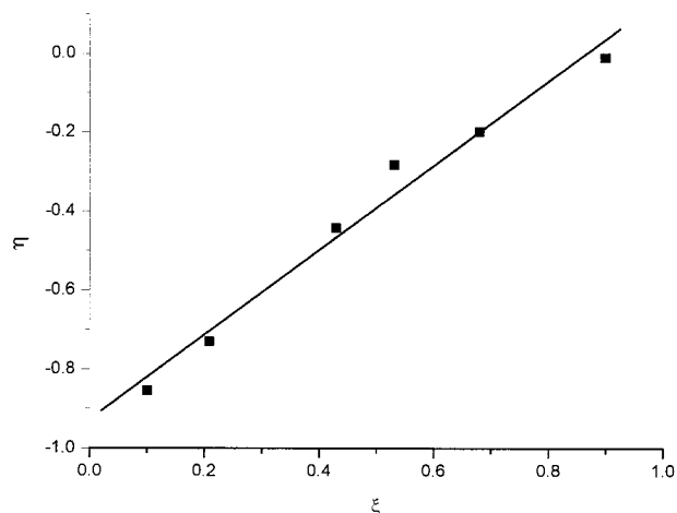
Figure 4 K-T method plot for determination of the monomer reactivity ratios of D-120 and styrene ( \alpha = 1.89 ).
