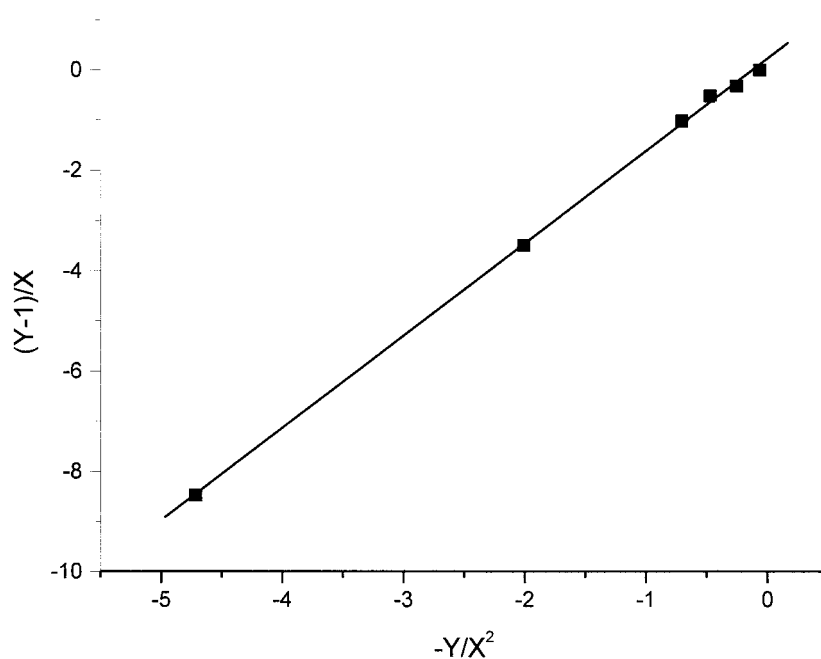
Figure 5 Fineman-Ross method for determination of the monomer reactivity ratios of D-120 and styrene.
